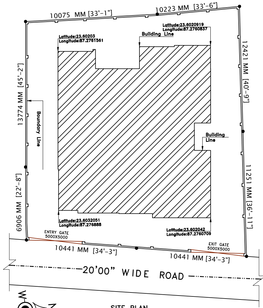
SITE PLAN
